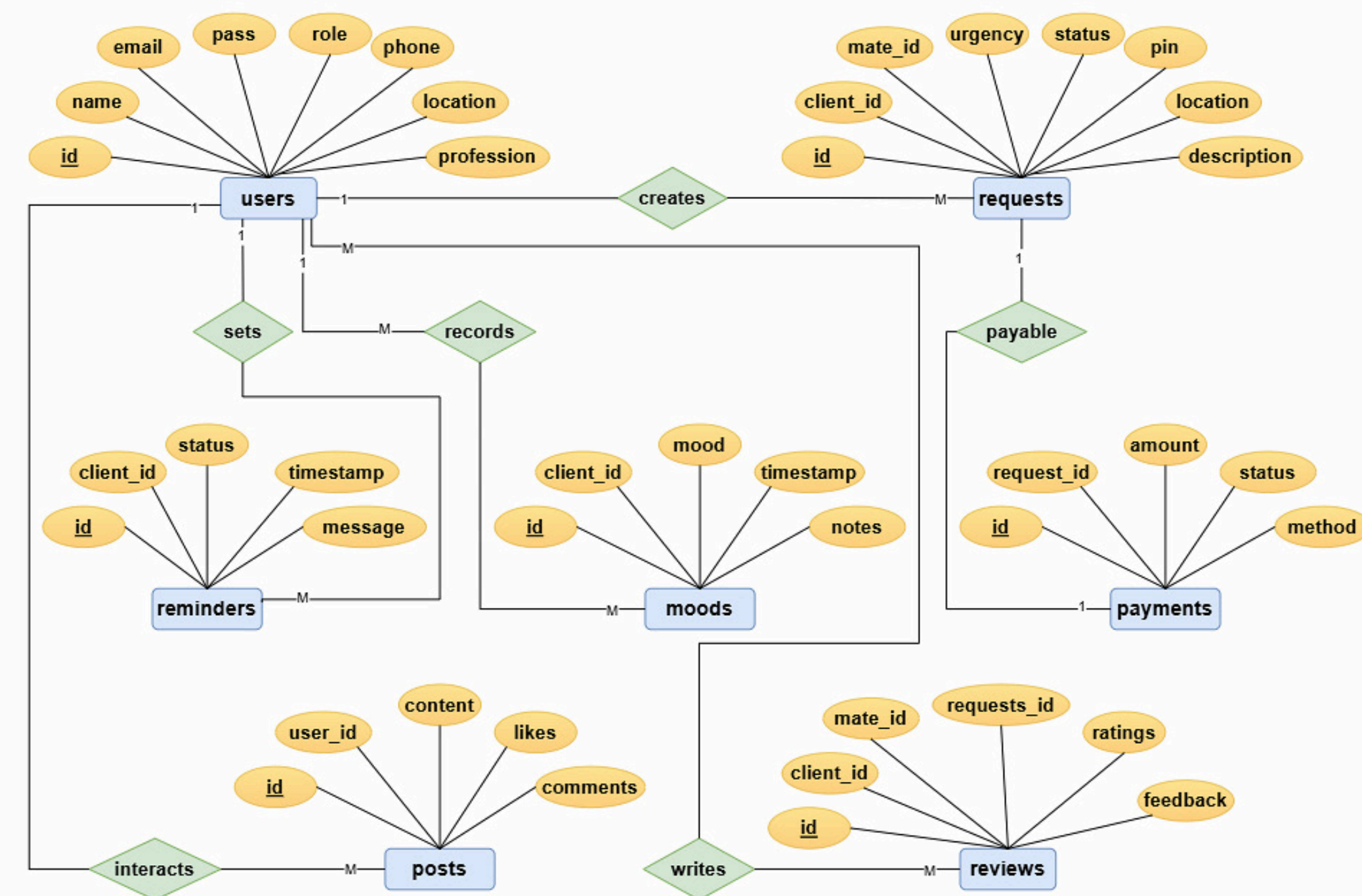
Fig-4: ER Diagram of CareConnect.
